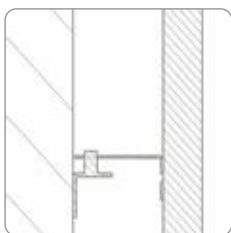
WALL SUSPENSION
